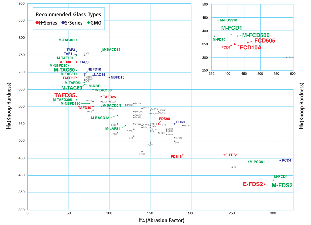
H_k - FA (Knoop Hardness-Abrasion Factor) Diagram
